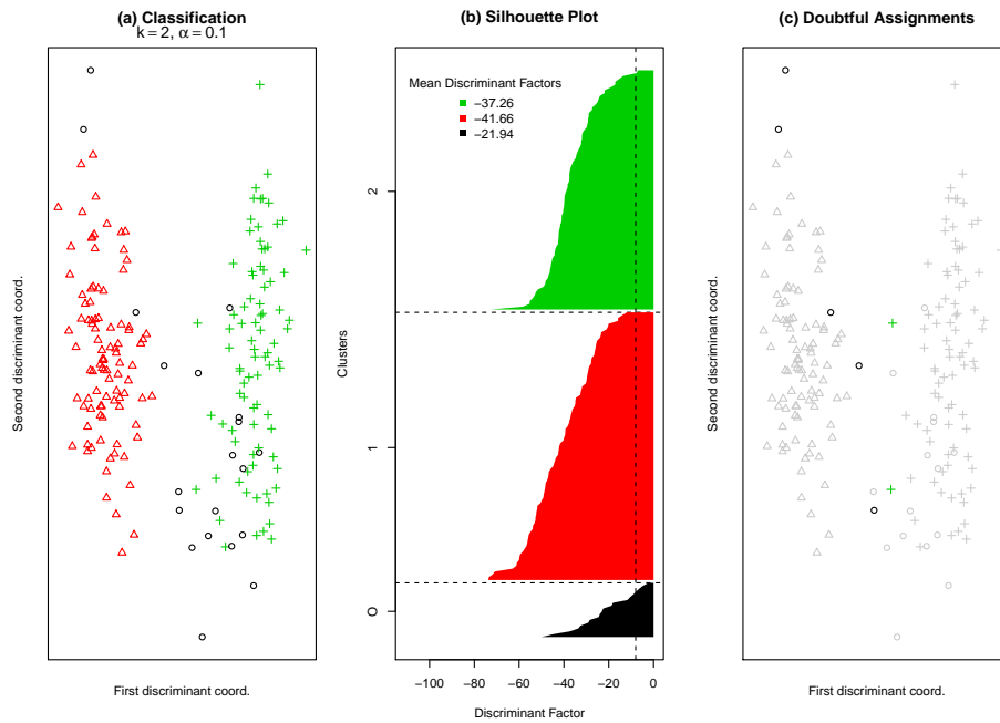
Figure 13: Clustering results with k = 2 , \alpha = 0.1 and restr.fact = 50 summarized by the use of DiscrFact function for the “Swiss Bank notes” data set. The threshold value is chosen in order to highlight the 7 most doubtful cluster assignments.
